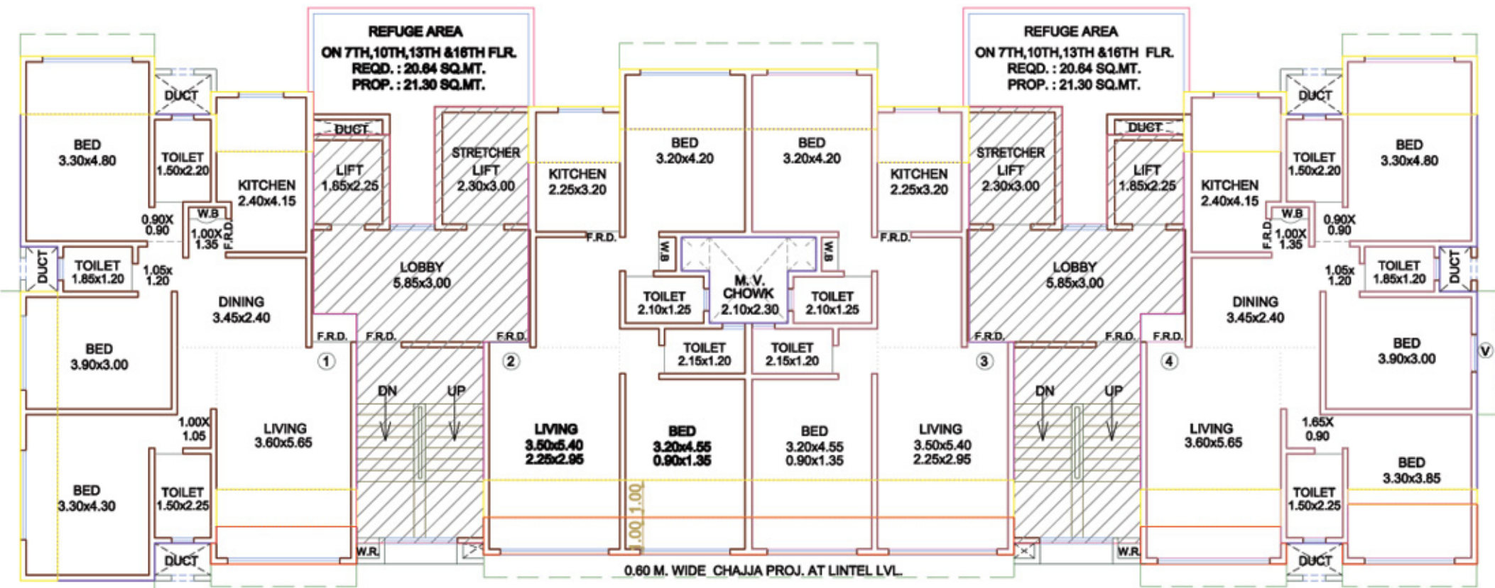
TYPICAL FLOOR PLAN (7TH TO 18TH) SCALE 1:100
